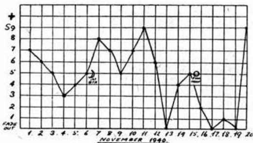
Observations on 19 metre transmissions from WGEA recorded by BRS3766.
